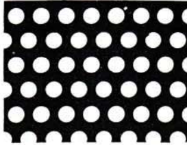
(9) 3.2 x 4.8P 39%
