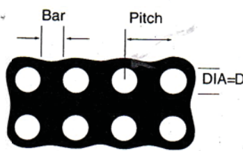
Square Pitch
