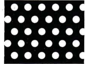
(8) 3.0 x 6.0P 23%
