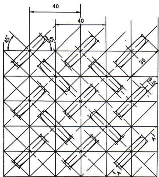
TOP VIEW DRAWING OF ANTI-SLIPPAGE BOARD LAYOUT
